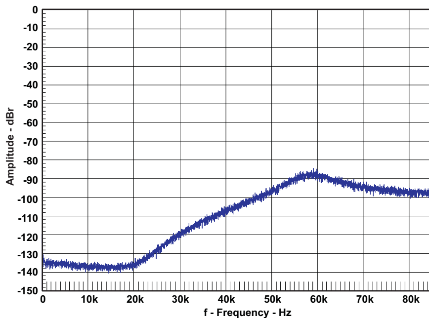
Figure 14. Idle Noise FFT Spectrum (SE)
