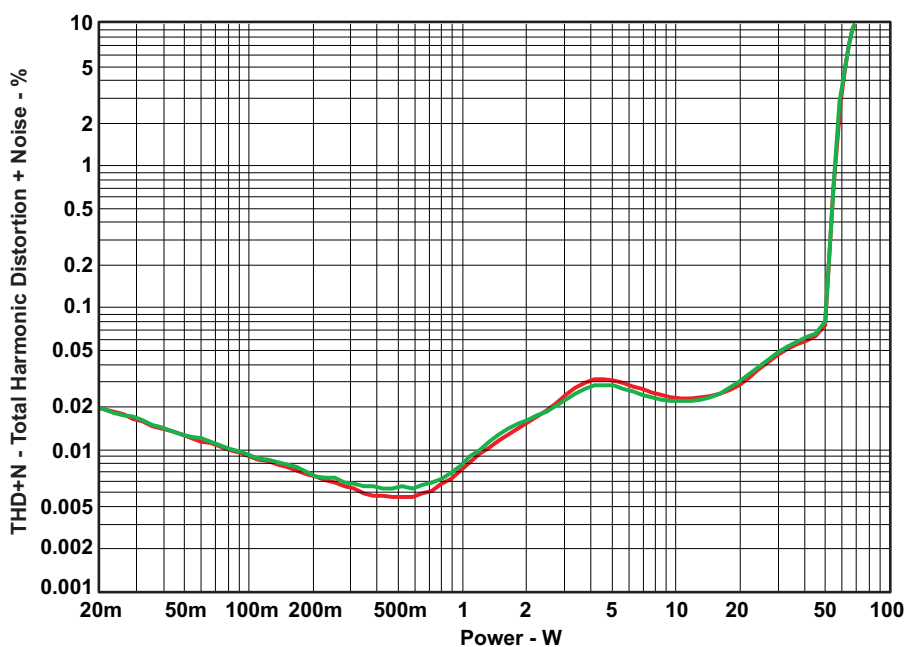
Figure 7. THD+N vs Power (BTL -8\ \Omega )
