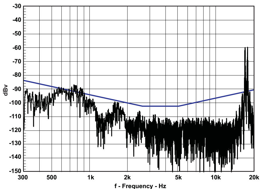
Figure 21. Pop/Click (SE)
