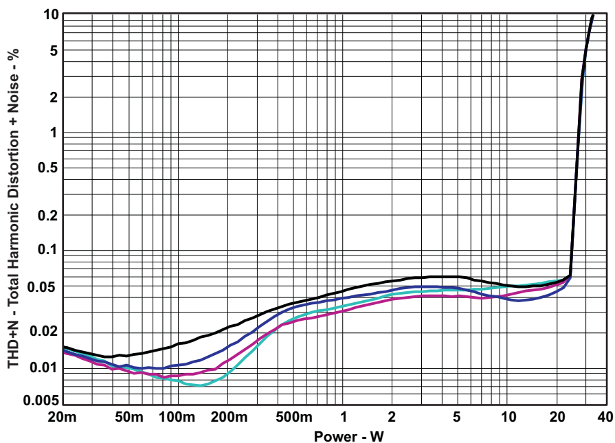
Figure 5. THD+N vs Power (SE -4\ \Omega )
