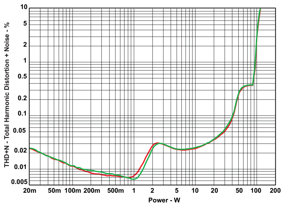
Figure 6. THD+N vs Power (BTL -4\ \Omega )
