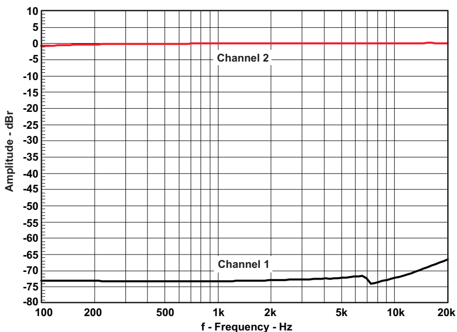
Figure 16. Channel Separation
