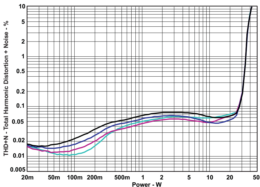
Figure 4. THD+N vs Power (SE -3\ \Omega )
