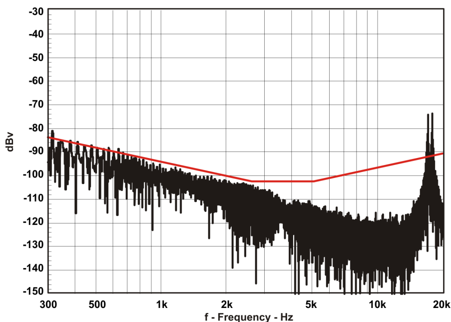
Figure 22. Pop/Click (BTL)
